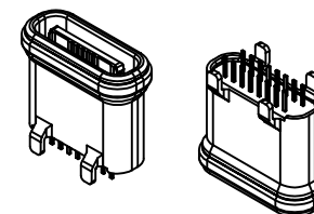
NO PART Q'TY Material 1 SHELL 1 ZINC ALLOG,Ni30u"Min PLATED 2 CONTACT 16 C7025,TiN80u"/Au3u"/Ni30u"PLATED 3 MID PLATE 1 SUS301,NO PLATING 4 HOUSING 1 LCP(E130i) UL94 V-0 BLACK 5 CAP 1 LCP UL94 V-0 BLACK 6 WATERPROOF RING 1 SILICONE(SI/60-65A) UL94 V-0 BLACK
